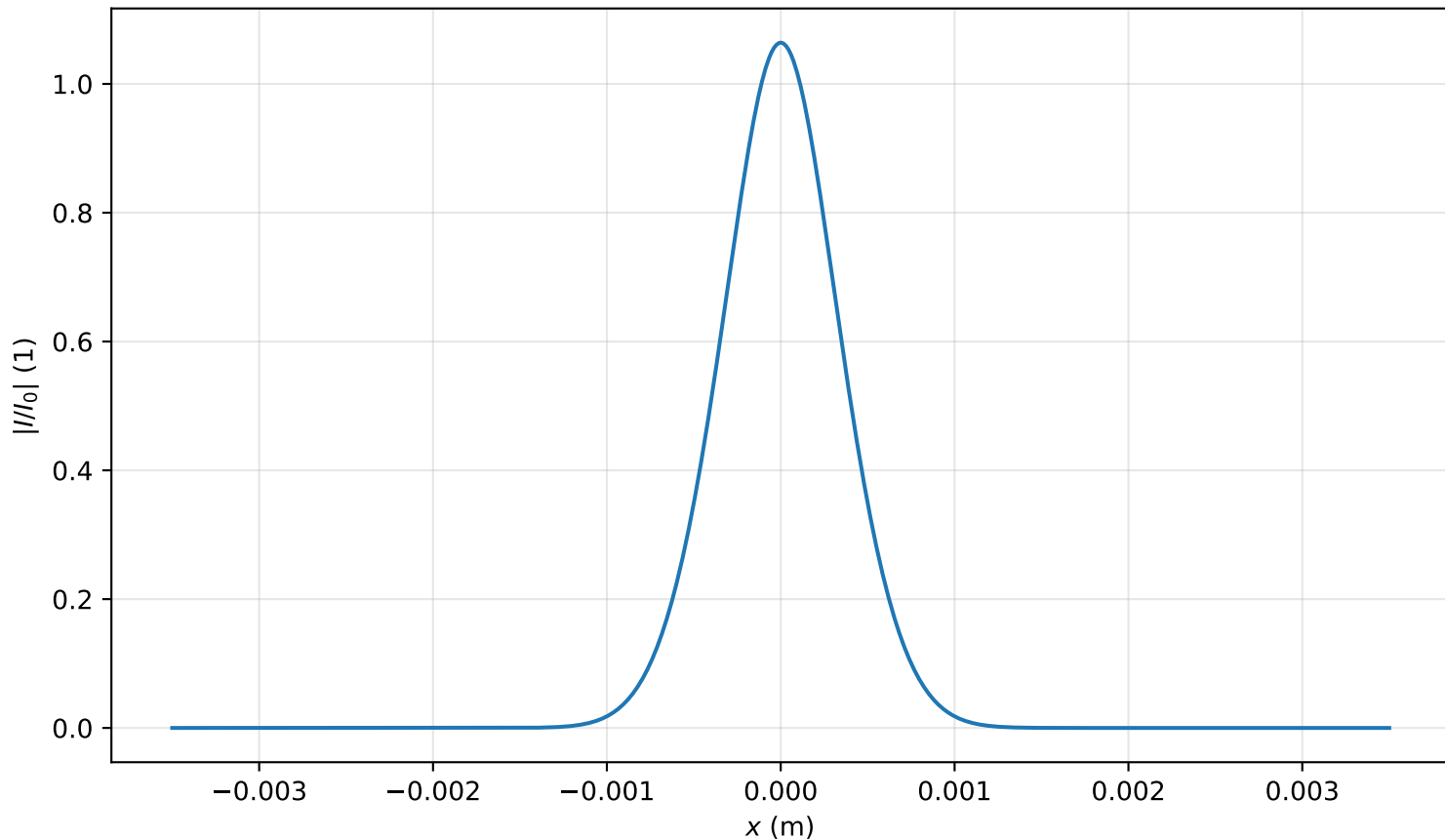
Intensity profile I(x, y = 0, z = 0.318m)/I_0 , P_{in}=0.9P_{cr} , artificial time
